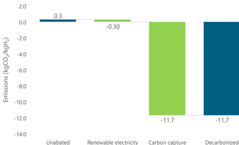
Figure 4-14 Emissions reduction – Gasification (Biogenic feed)
