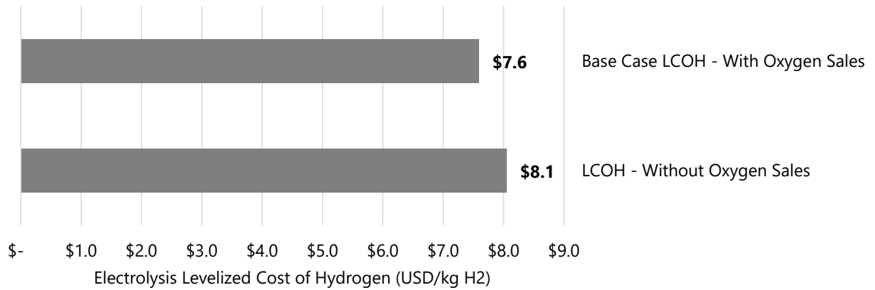
Figure 5-5 LCOH Electrolyzer Oxygen Revenue Sensitivity Cases
