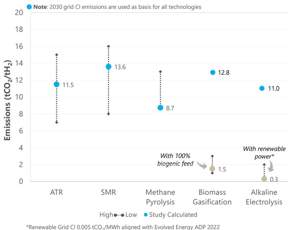
Figure 6-1 Calculated unabated emissions comparison to literature
