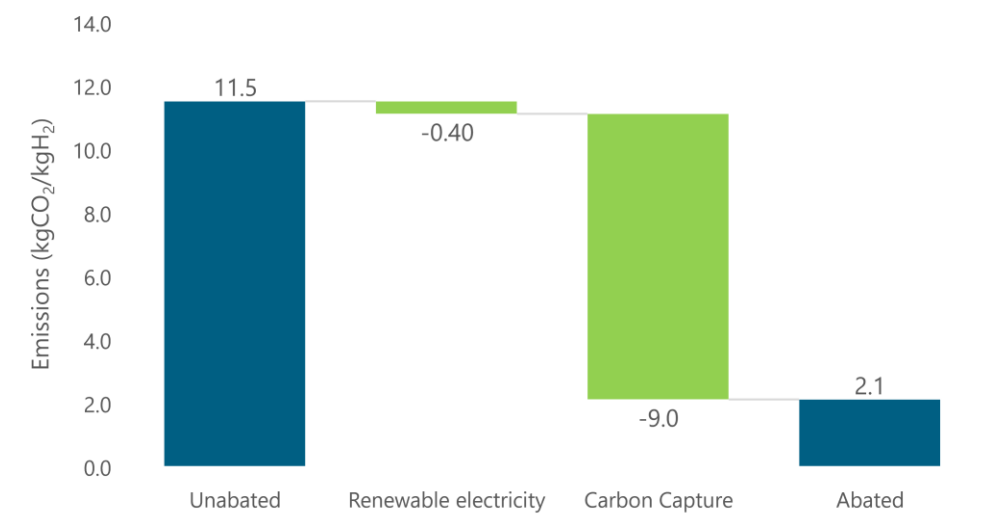
Figure 4-7 Emissions reduction – ATR
