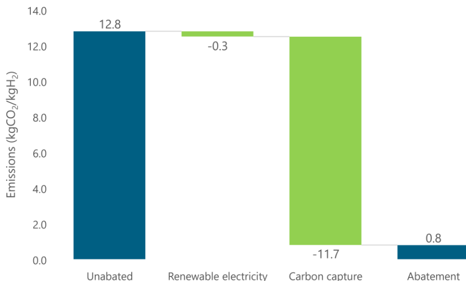
Figure 4-13 Emissions reduction – Gasification (Non-biogenic feed)
